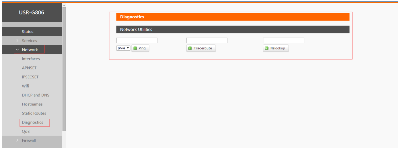
Figure 28 Network diagnosis
