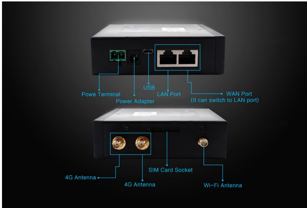
Figure 3 Interface
