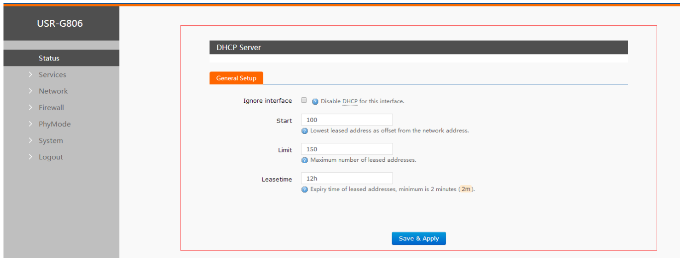
Figure 21 DHCP function
