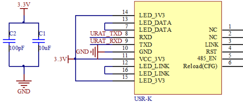
Diagram 4-4 Hardware to RJ45 light
