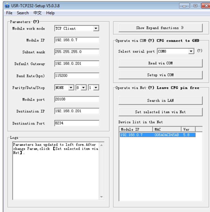
Diagram 3-3 TCP Client
