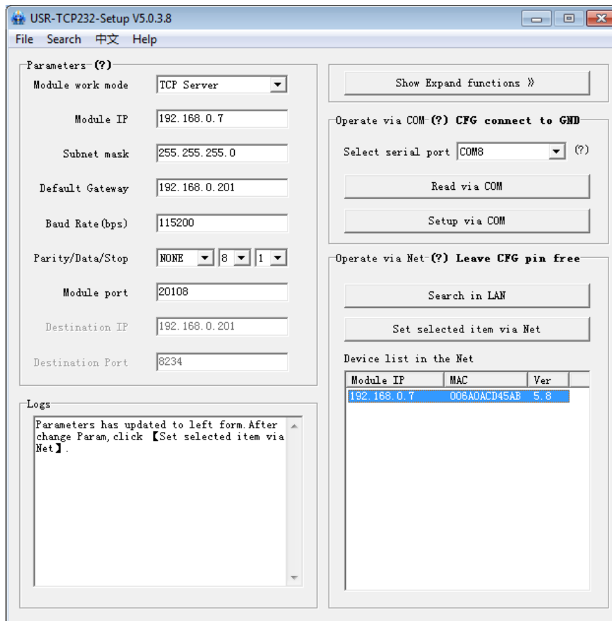
Diagram 3-5 TCP Server Mode
