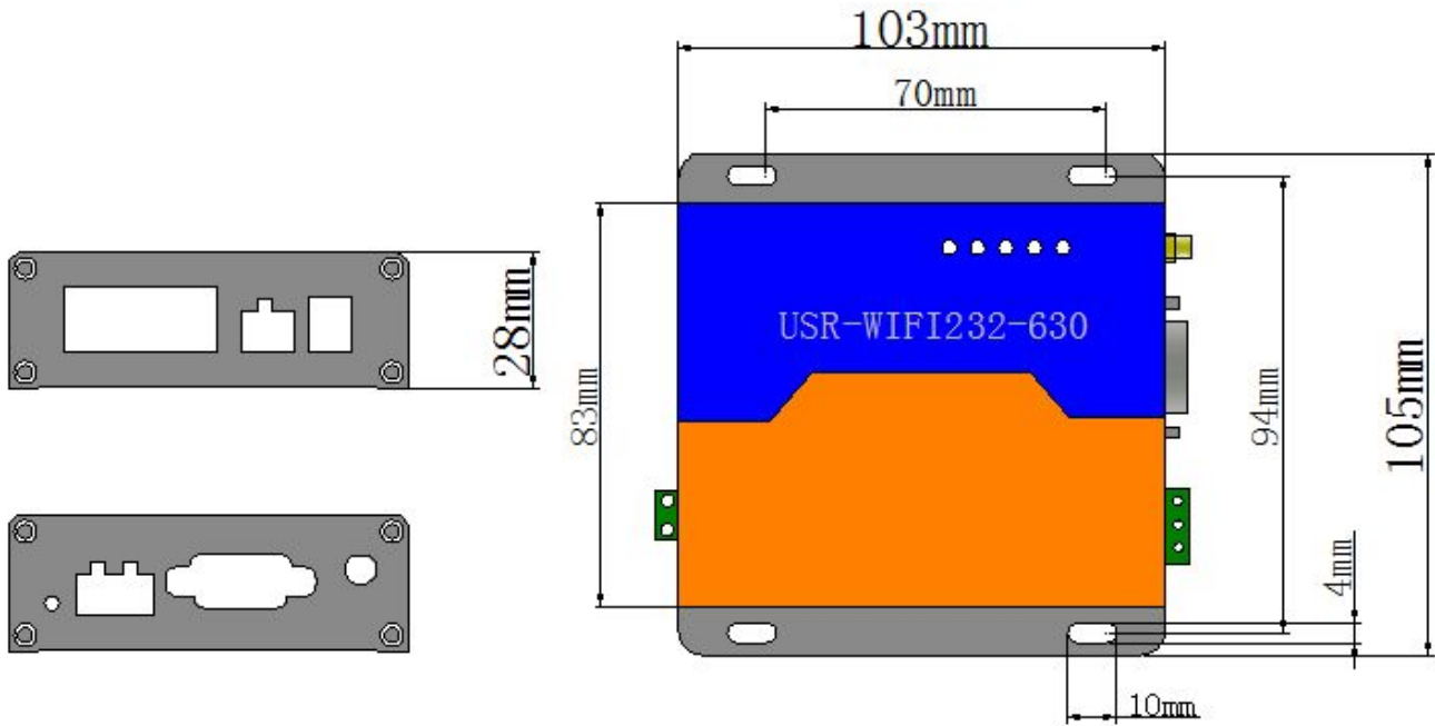
Figure 5 Appearance size chart(602/604/610)
