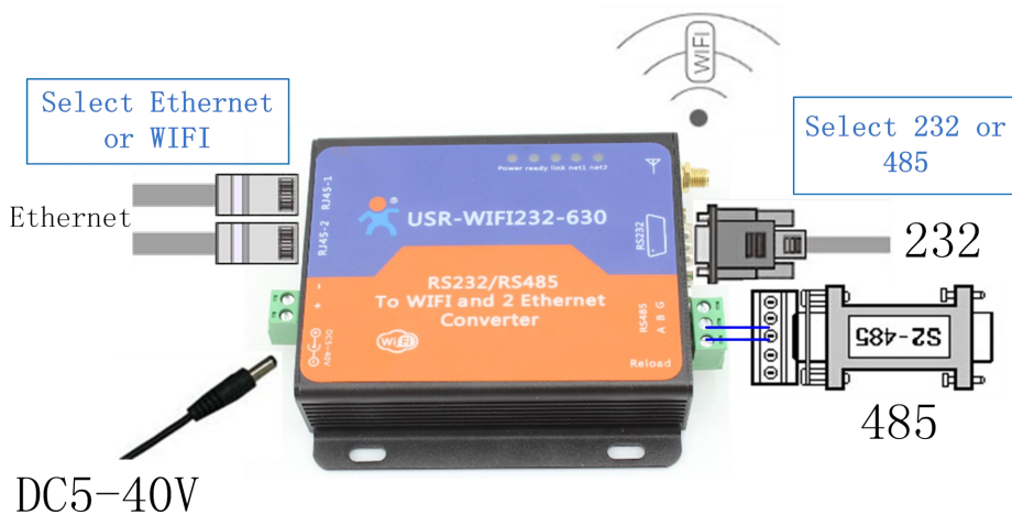
Figure 1 Hardware Connect
