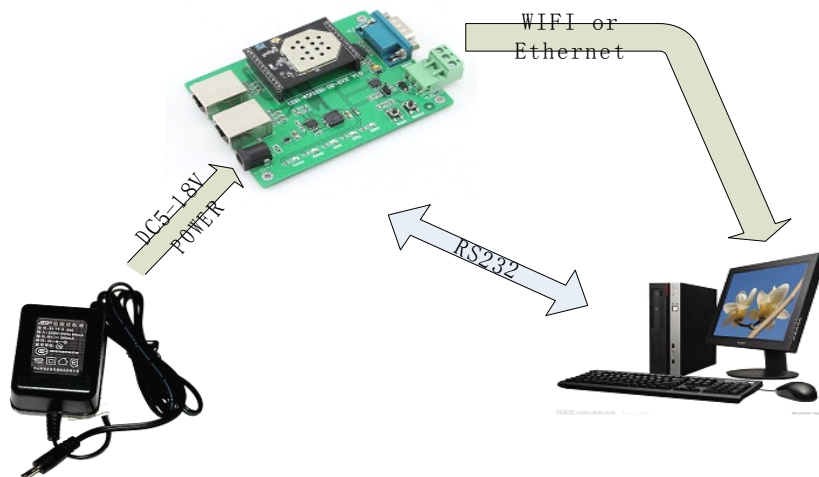
Figure 46 Connection diagram
