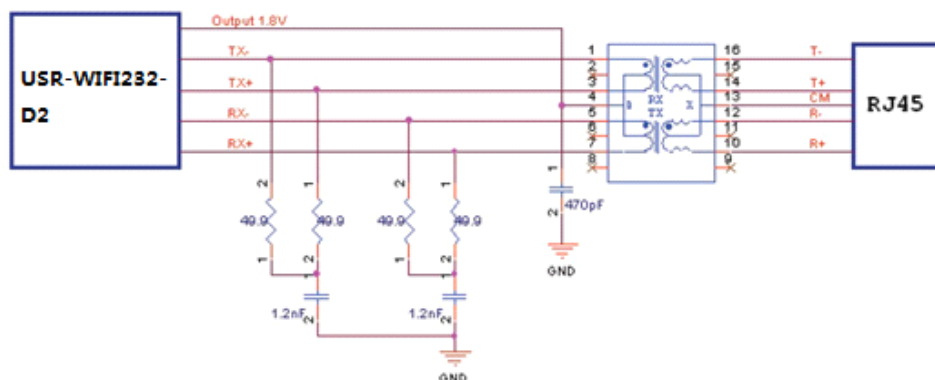
Figure 16 Ethernet Reference Design with Transformer
