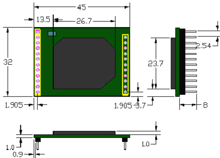
Figure 10 USR-WIFI232-D2 Mechanical Size
