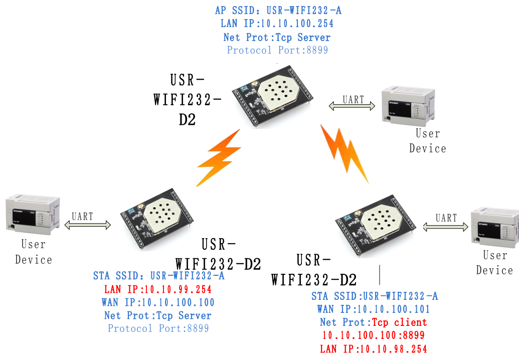
Figure 61 Two USR-WIFI232-D2 Modules Connection Through AP
