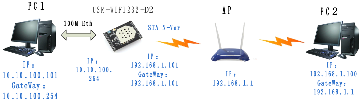
Figure 23 USR-WIFI232-D2 Ethernet Interface Networking (As STA, N-Ver)
