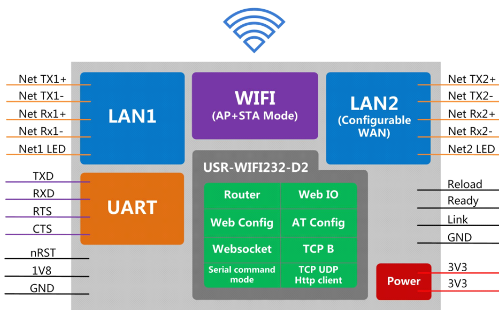
Figure 5 Block diagram
