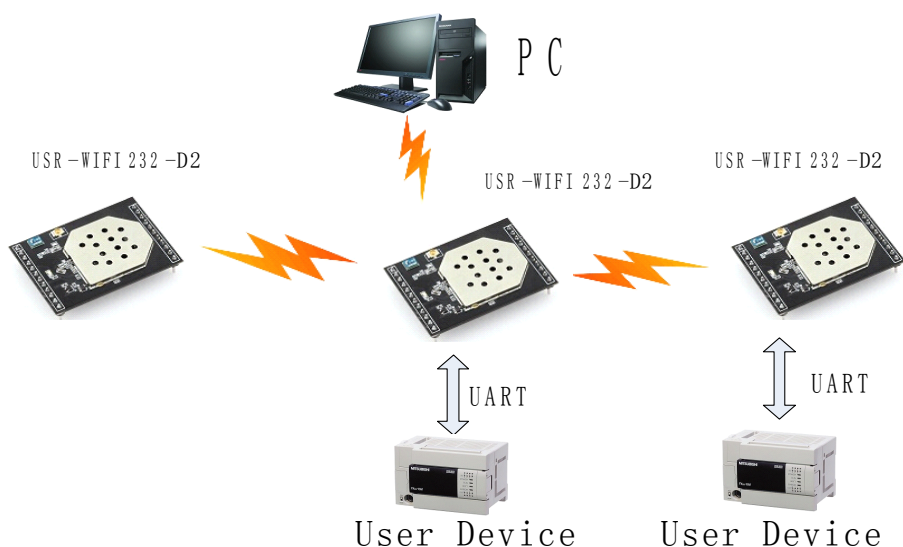
Figure 20 USR-WIFI232-D2 STA Network Structure
