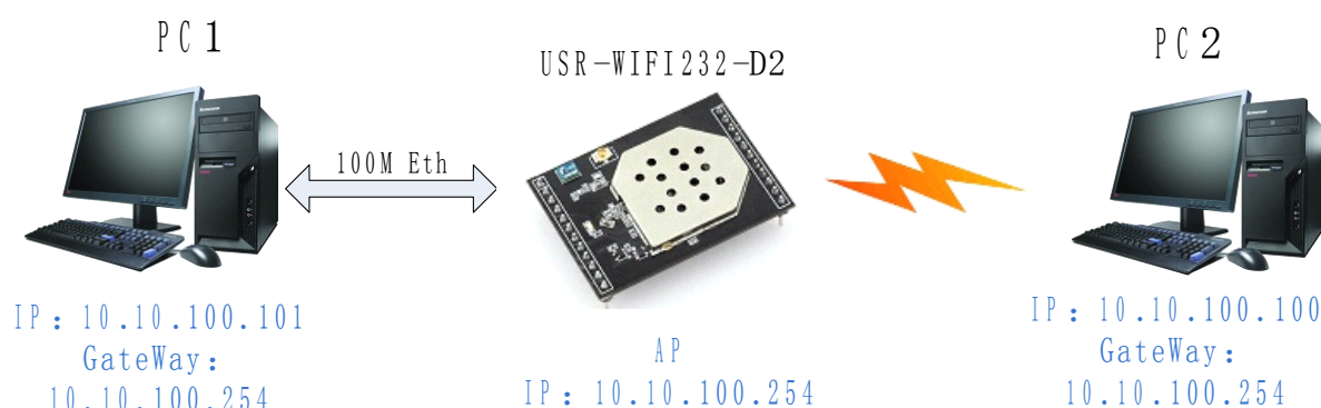
Figure 22 USR-WIFI232-D2 Ethernet Interface Networking (As AP)
