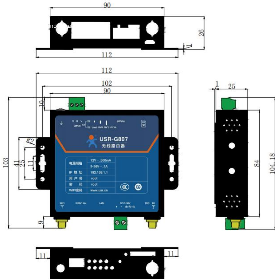
USR-G807 Dimensions
