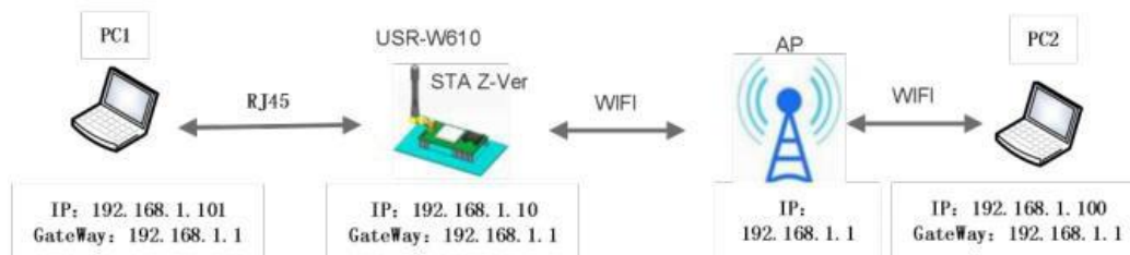
Figure 8. Bridge Mode
