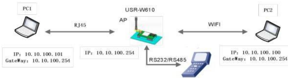
Figure 6. AP+ALN Application
