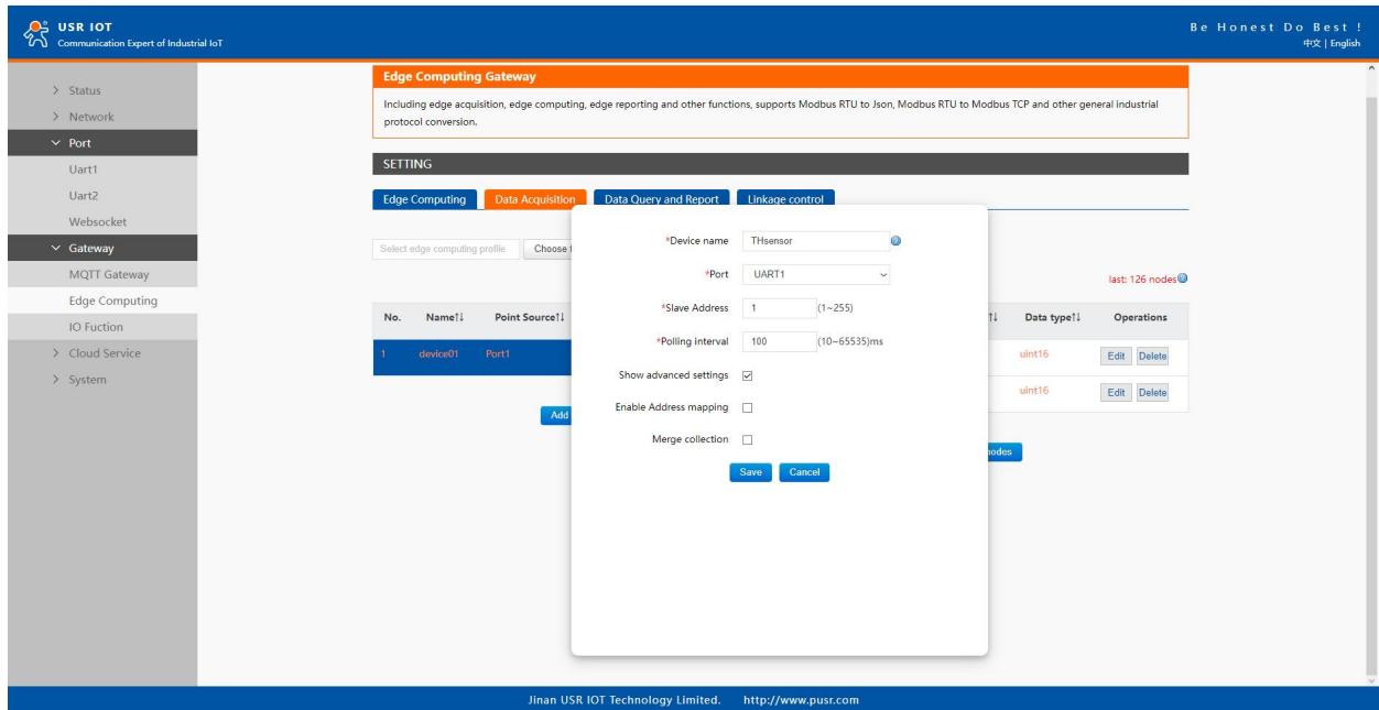
Fig. 34 Polling slave device configuration
