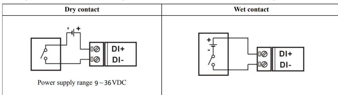
Fig. 3 Dry/Wet contact wiring
