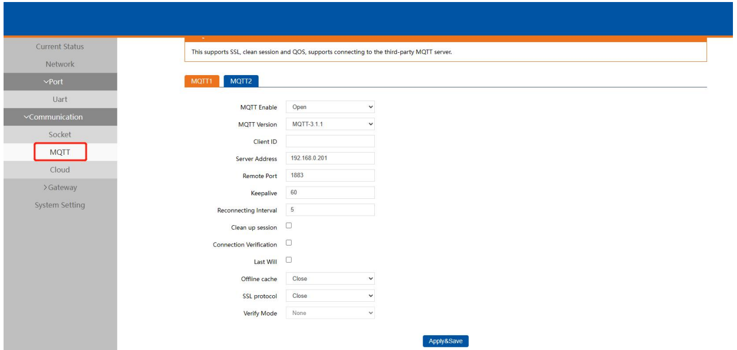
Fig. 19 MQTT connection profiles
