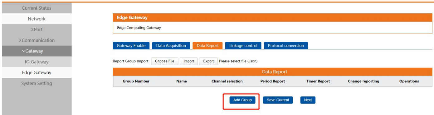
Fig. 25 Data report
