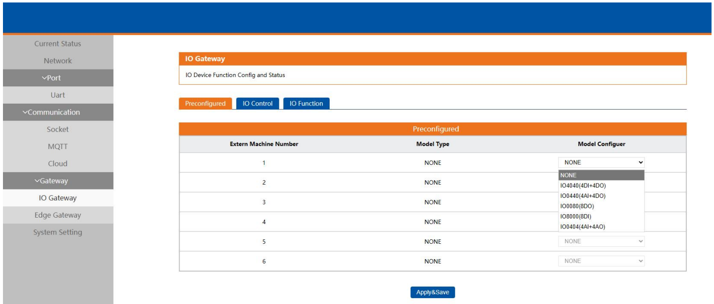
Fig. 20 Preconfigured Page
