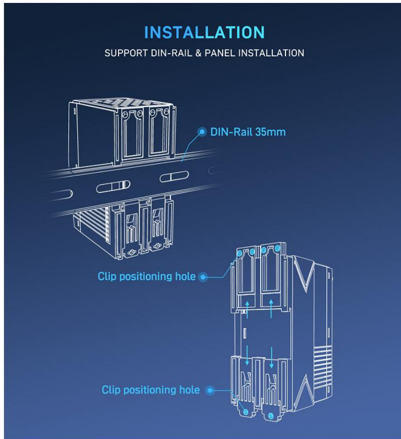
Fig. 1 DIN-Rail mounting and wall mounting
