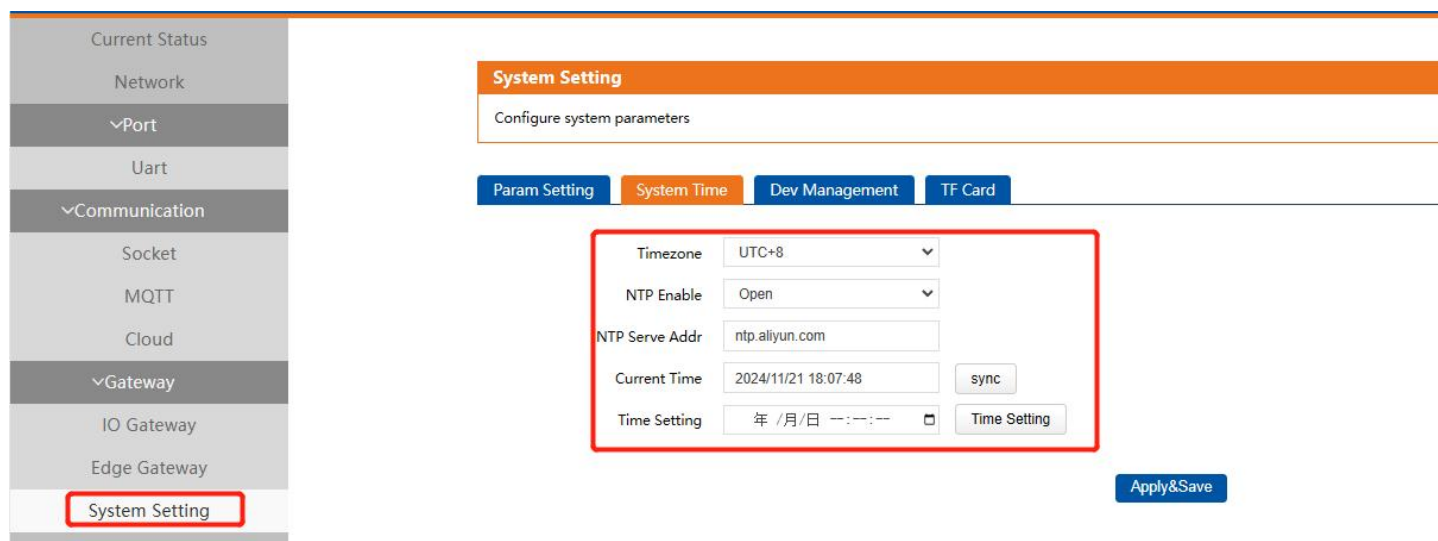
Fig. 28 System time
