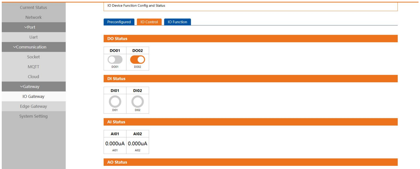
Fig. 21 IO control
