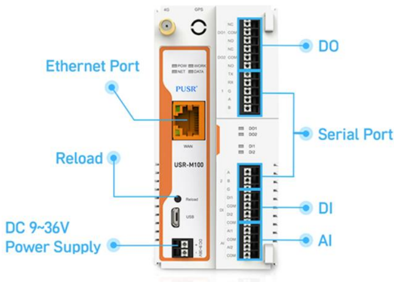
Fig. 2 USR-M100-HM interfaces
