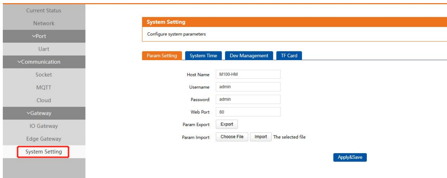
Fig. 27 System settings
