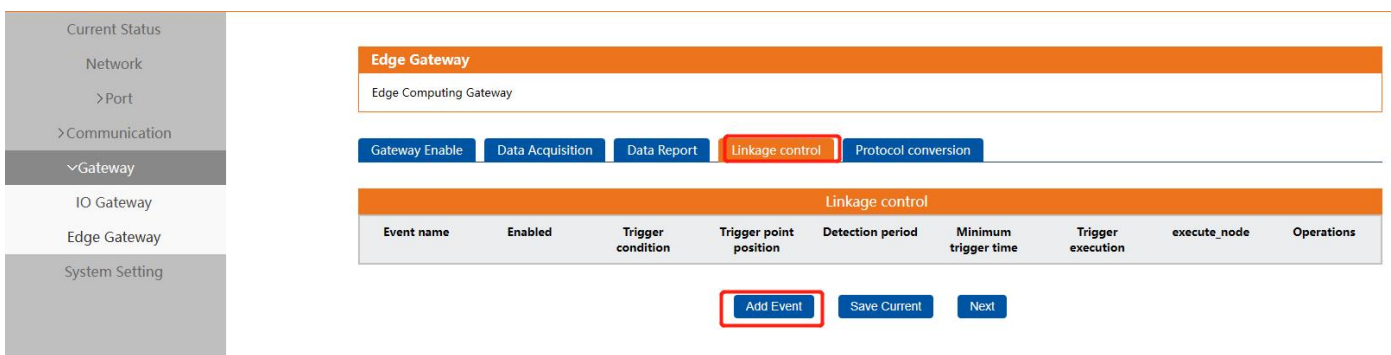
Fig. 26 Linkage Control
