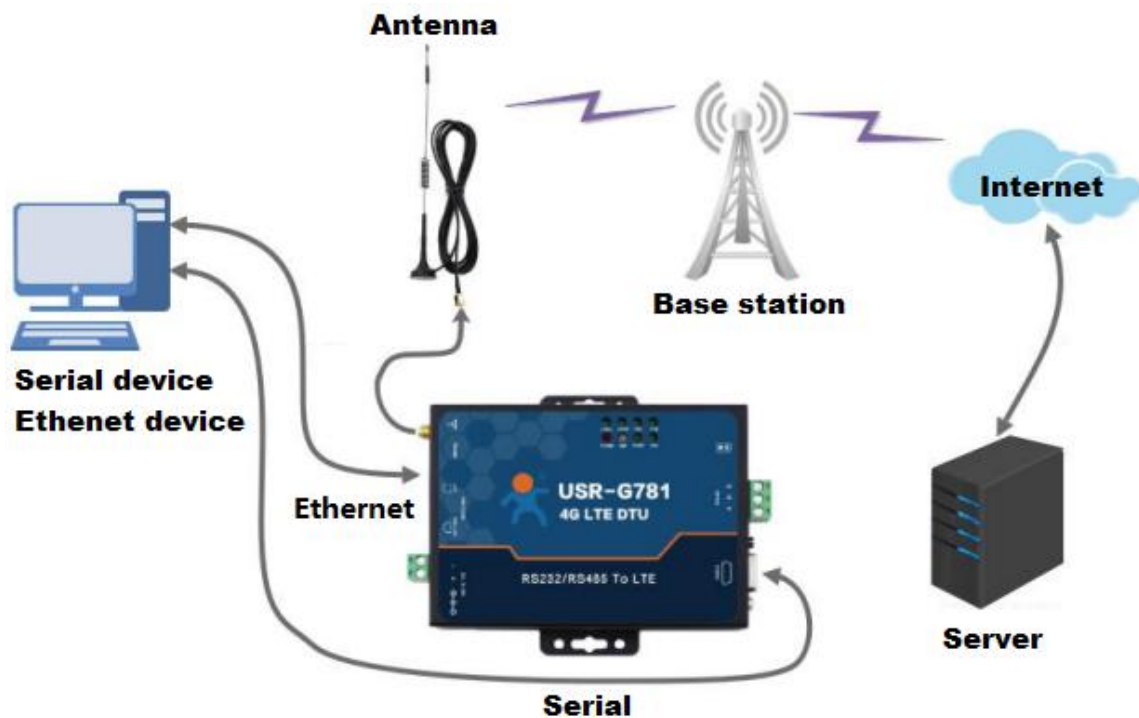
Figure 2 Application diagram
