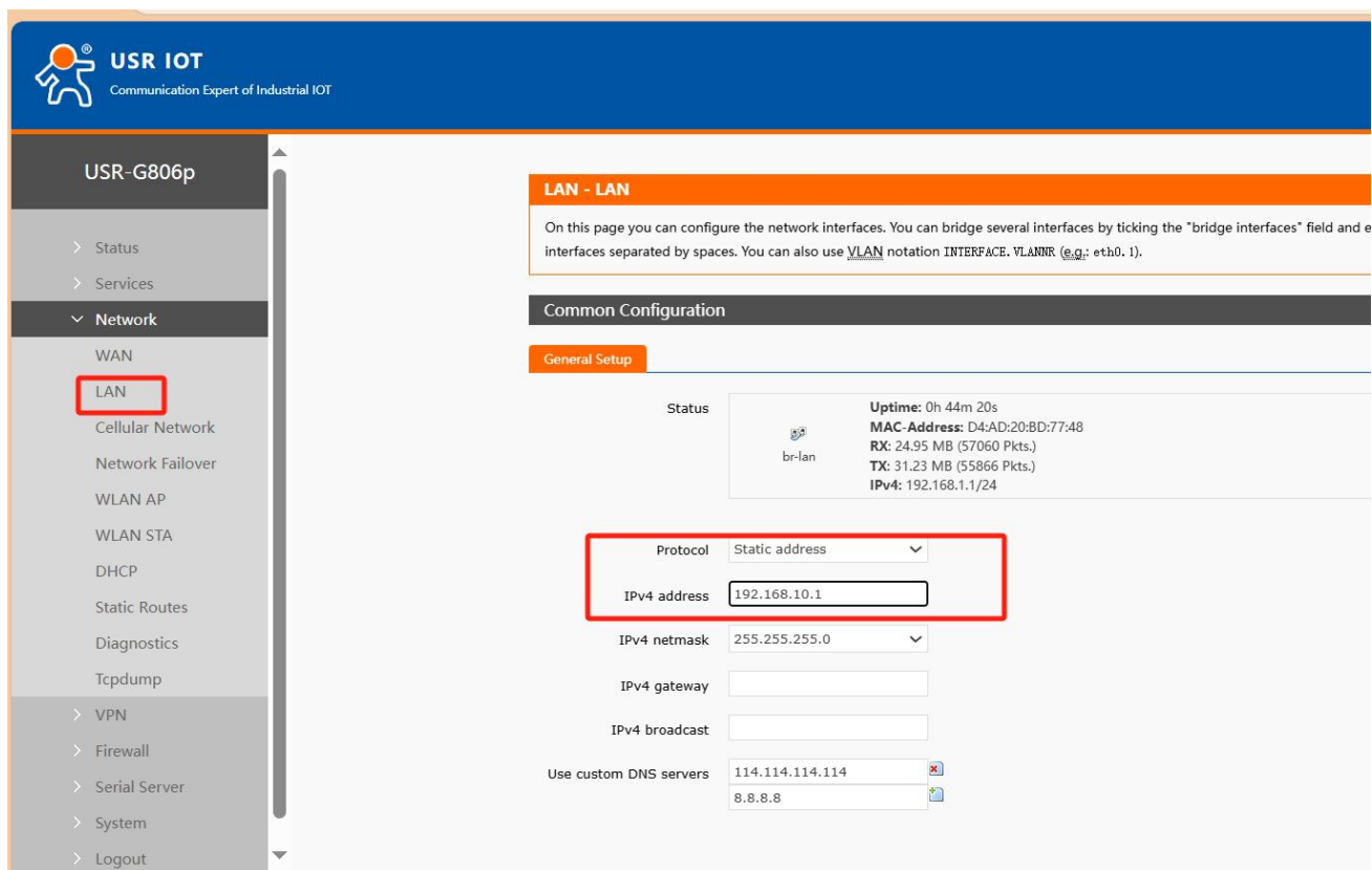
Pic 43 Router 1 is configured 1
