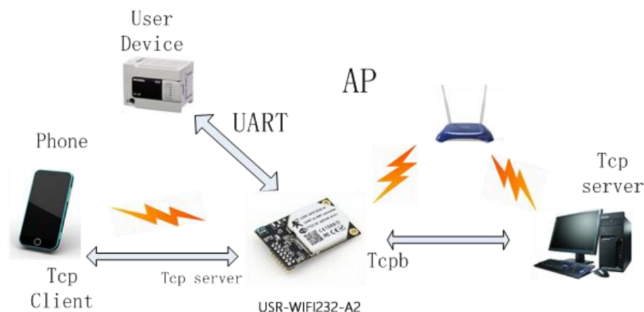
Figure 18 USR-WIFI232-A2 AP+STA Network Structure
