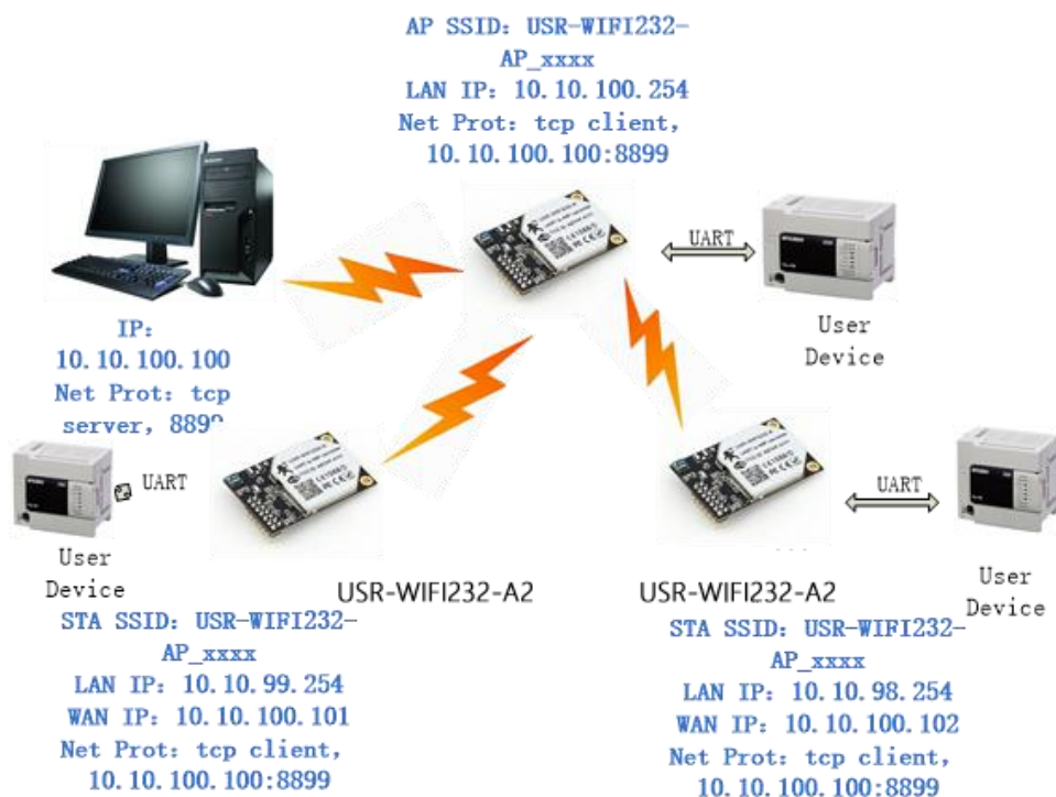
Figure 50 Wireless Data Acquisition Card Application
