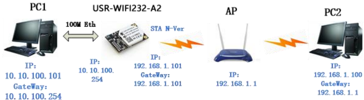
Figure 20 USR-WIFI232-A2 Ethernet Interface Networking (As STA, N-Ver)
