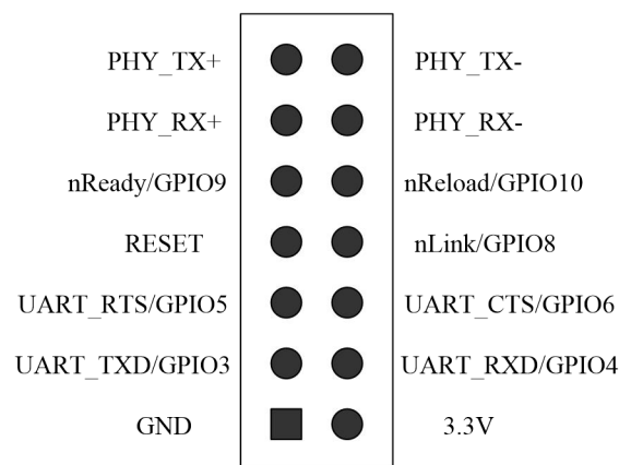
Figure 7 USR-WIFI232-A2 Pins Map
