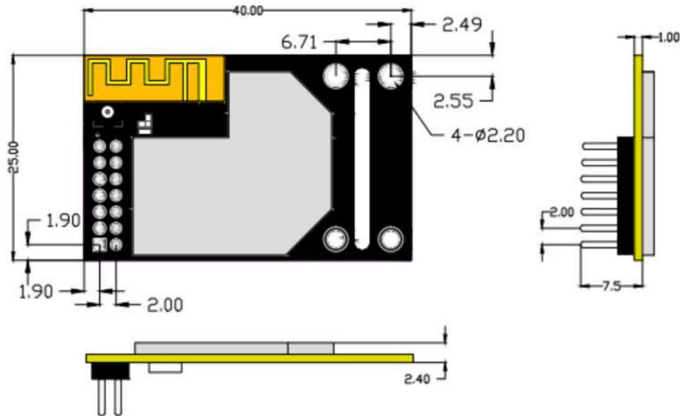
Figure 8 USR-WIFI232-A2 Mechanical Size
