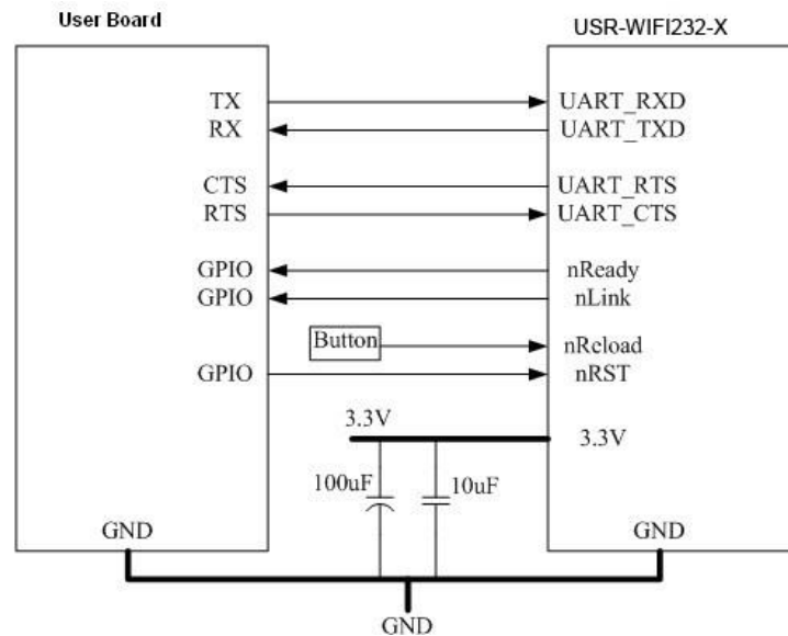
Figure 10 USR-WIFI232-A2 Hardware Typical Application
