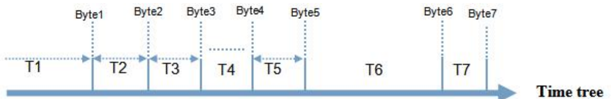
Diagram22 Switching command mode order
